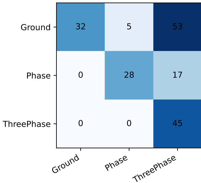
IEEE14 Baseline+NormVI
