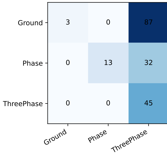
IEEE30 Baseline+NormVI
