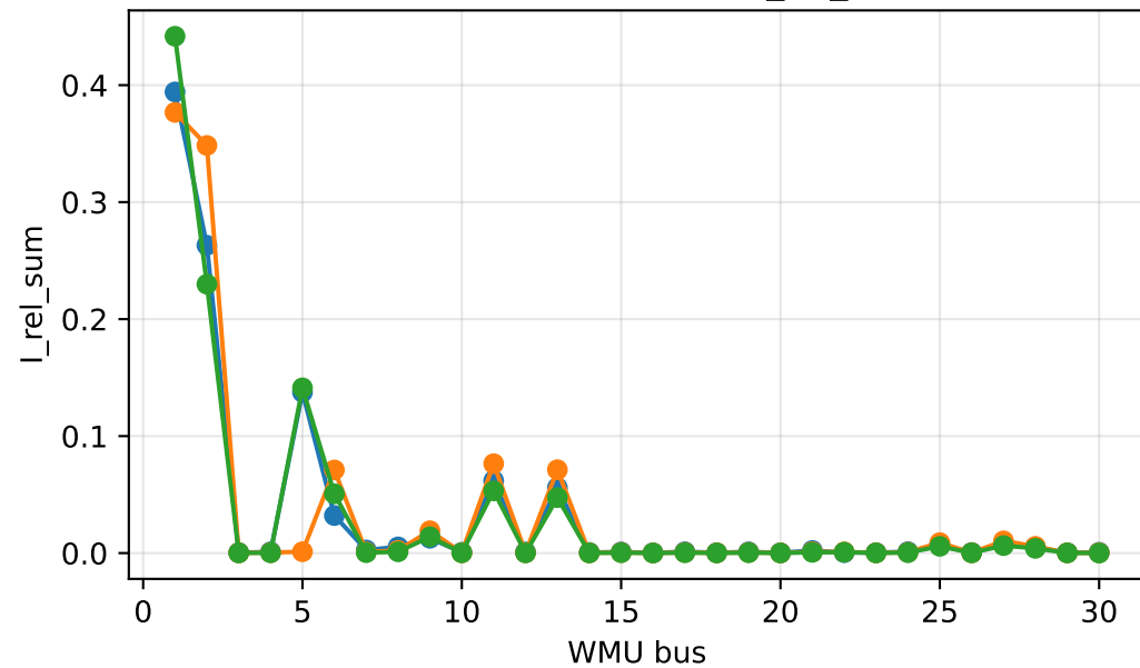
IEEE30 representative I_rel_sum
