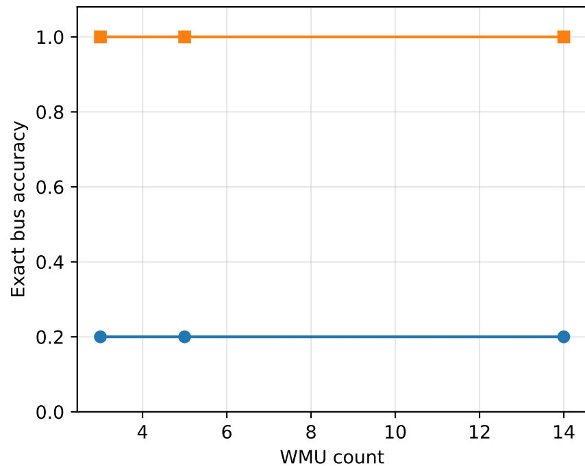
Reduced-WMU robustness under unseen 10\Omega
