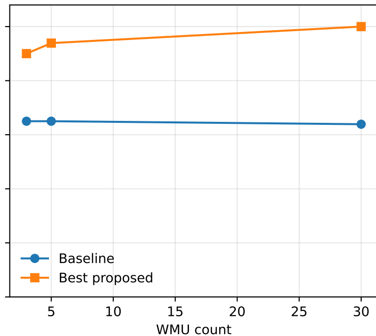
Reduced-WMU robustness under unseen 10\Omega
