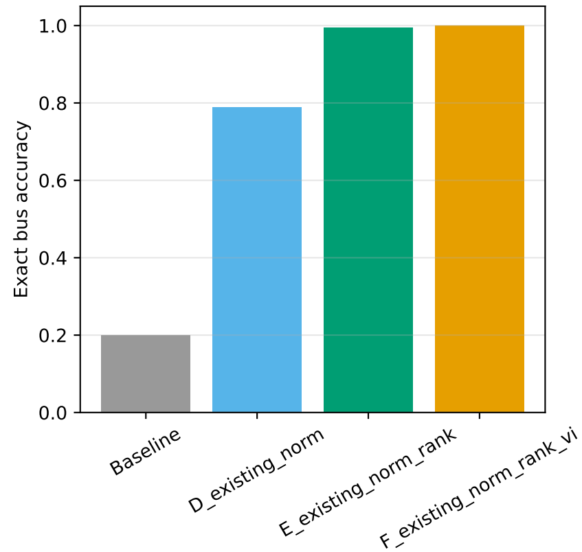
Baseline absolute features vs normalized spatial features ieee14 unseen 10 \Omega full-WMU
