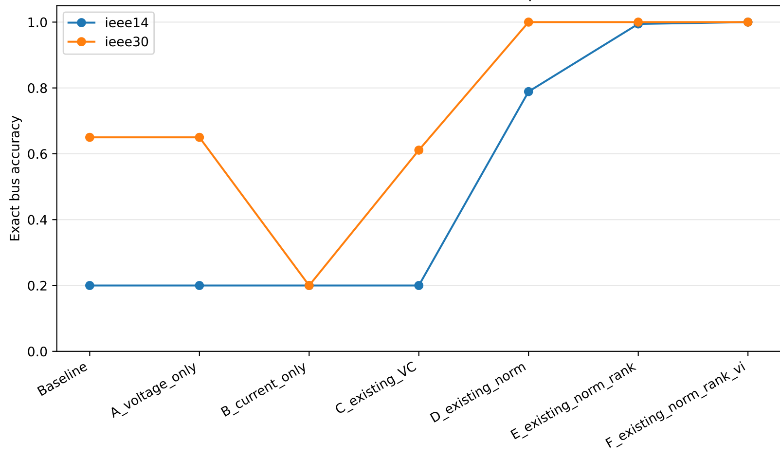
Feature ablation: absolute vs normalized/spatial features
