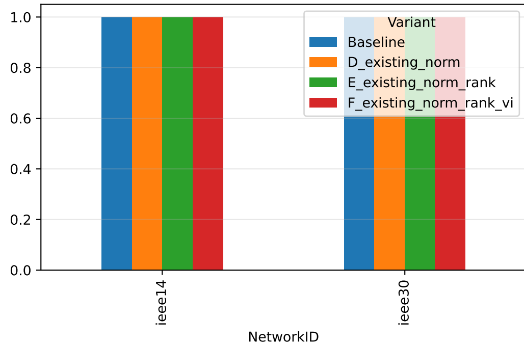
Fault detection recall @ 10 \Omega
