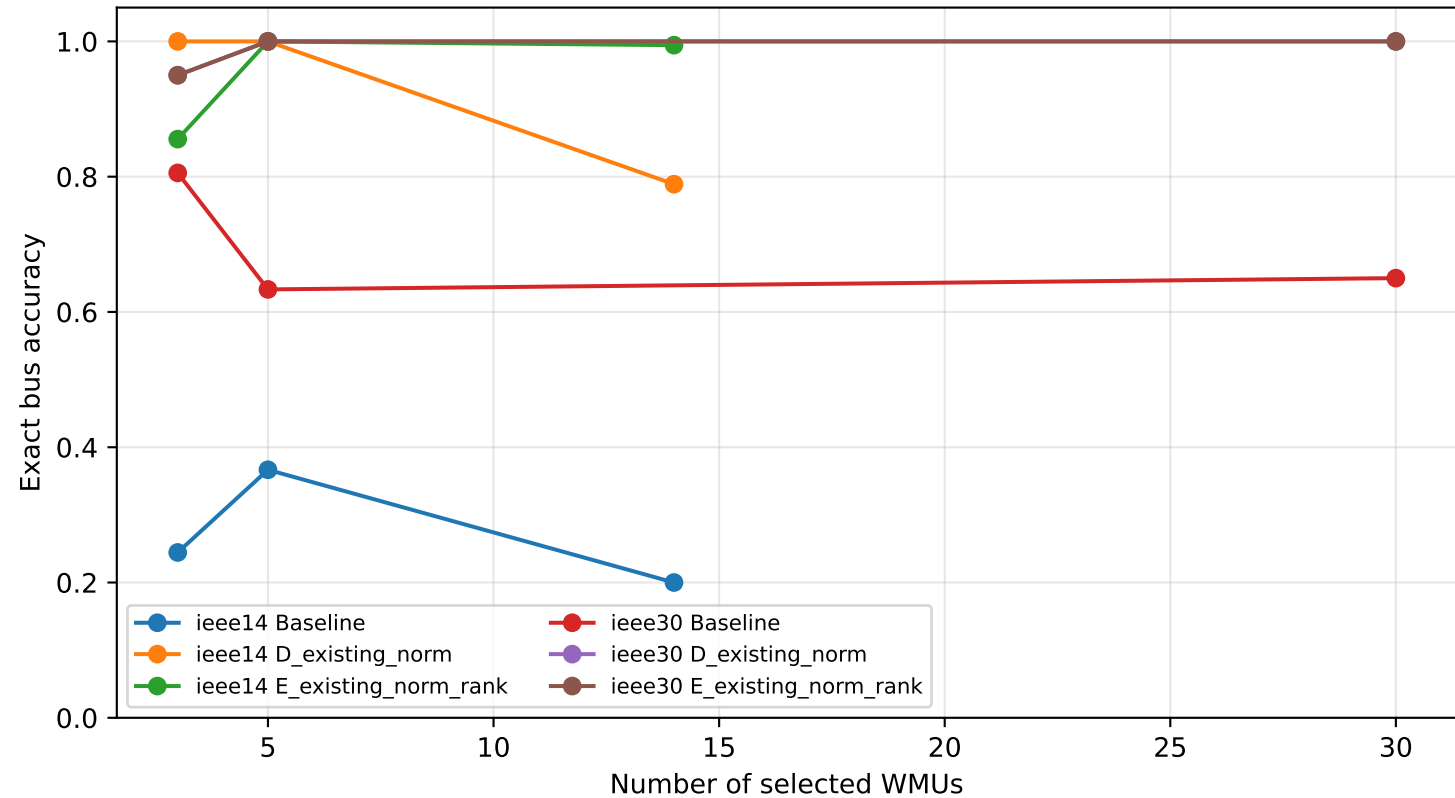
Reduced-WMU unseen 10Ω localization
