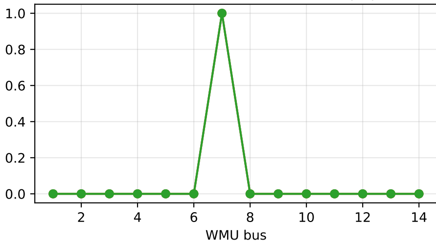
ieee14 bus 2 ThreePhase: Normalized |\Delta I| / \max
