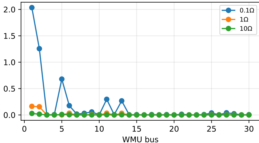
ieee30 bus 1 ThreePhase: Normalized |\Delta I| / \max
