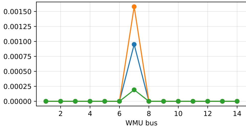
ieee14 bus 2 ThreePhase: Normalized |\Delta I| / \max
