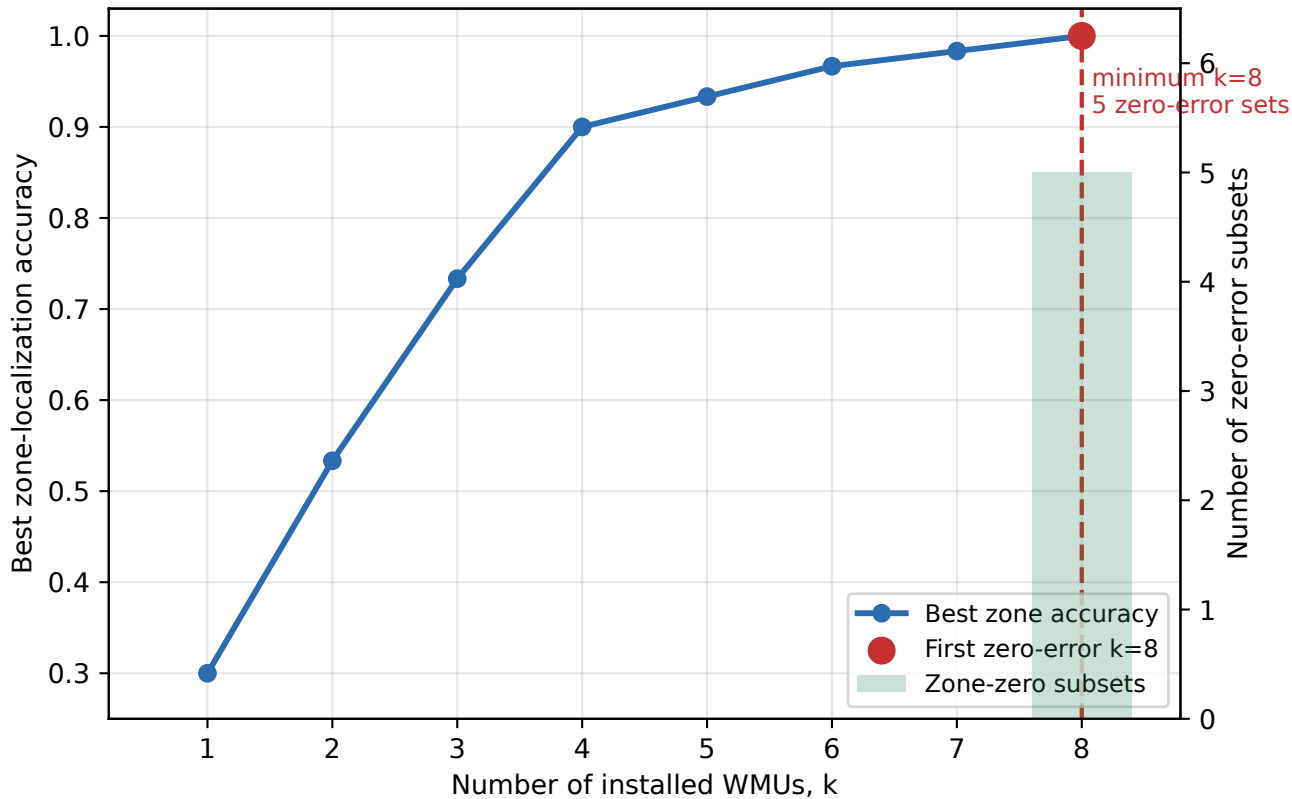
Fig. 3. Minimum WMU count for zone localization
