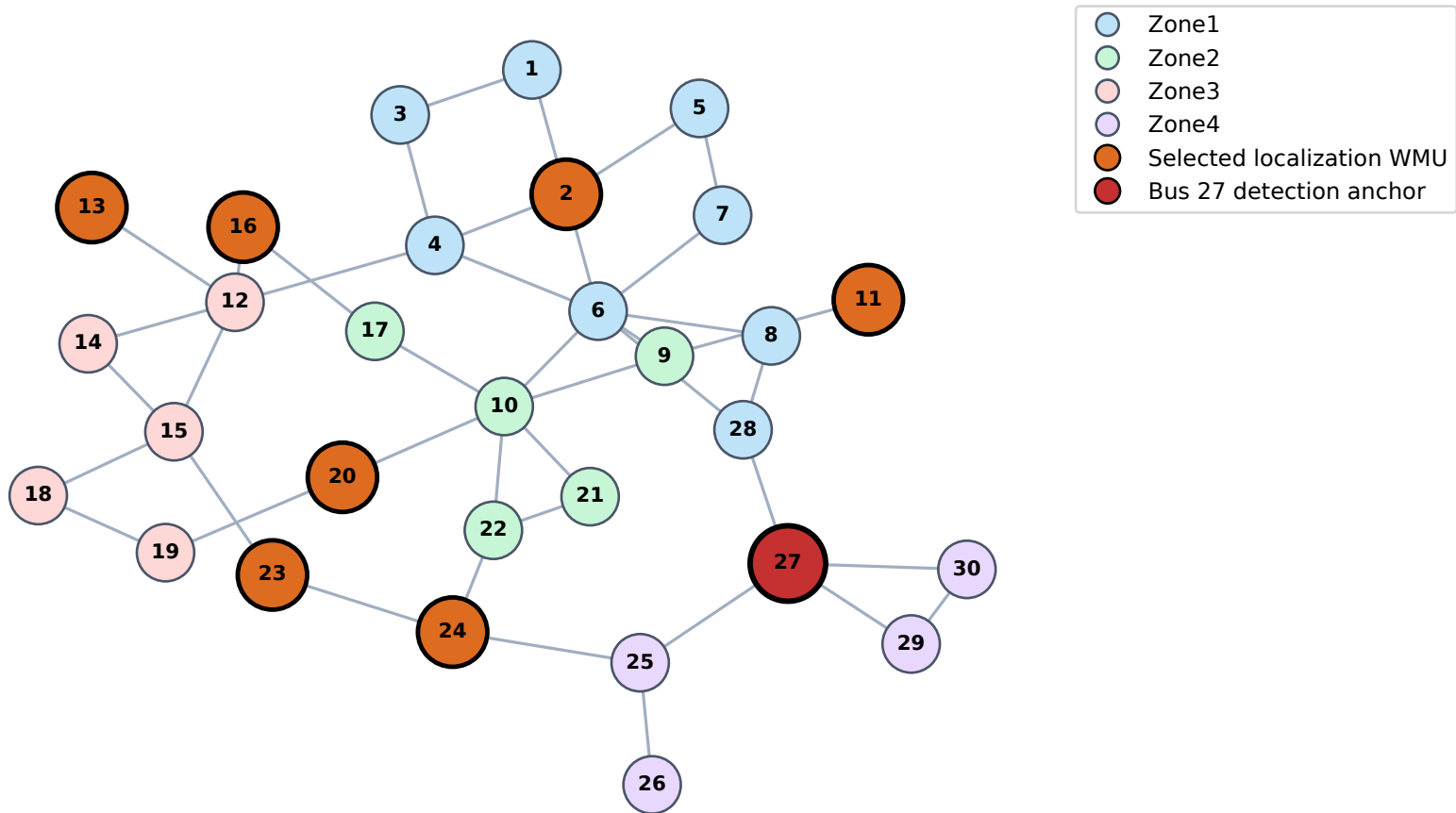
Fig. 4. Selected 8-WMU placement on IEEE 30-bus topology
