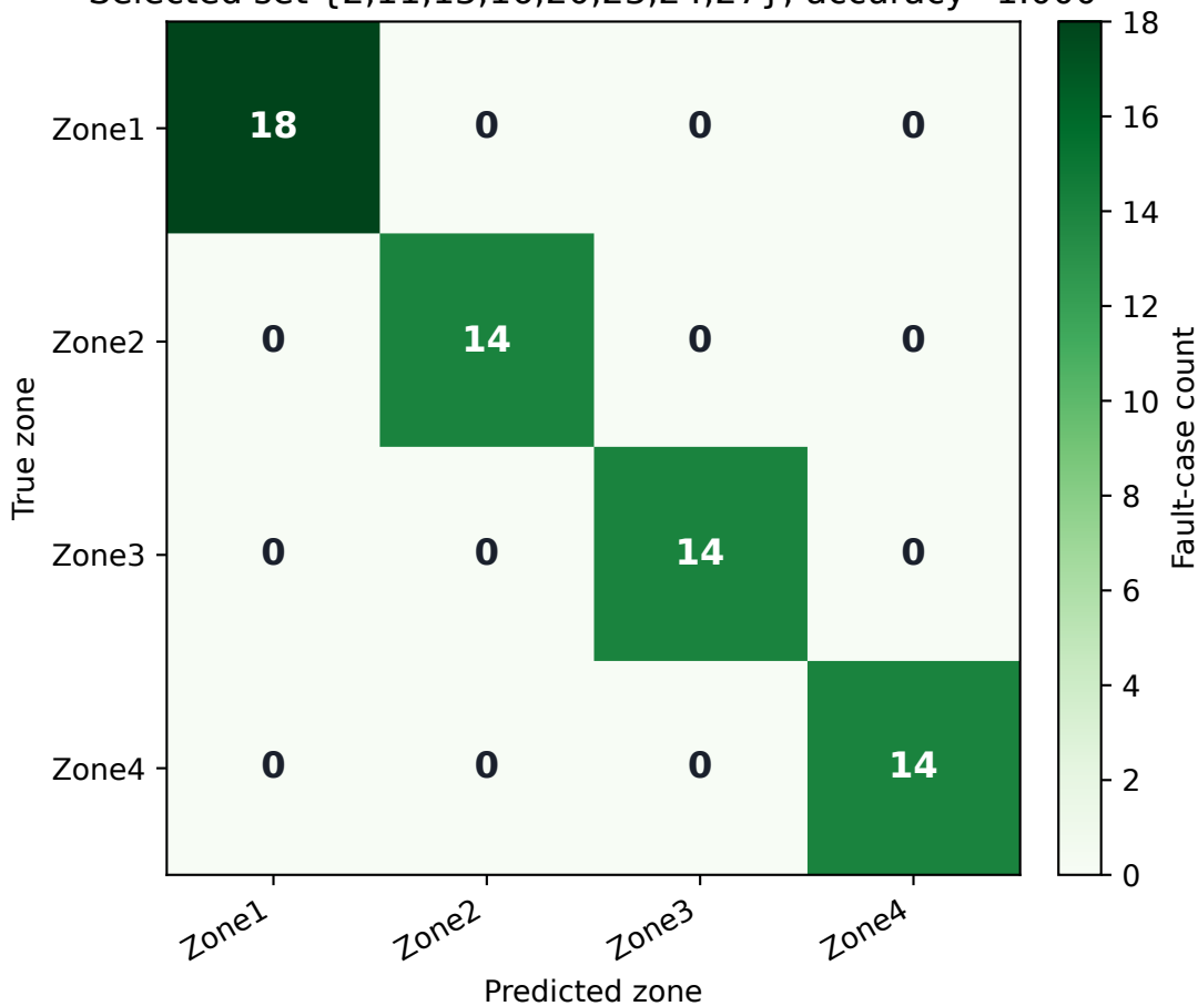
Fig. 5. Zone localization confusion matrix Selected set {2,11,13,16,20,23,24,27}; accuracy=1.000
