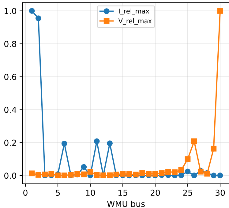
ieee30 representative CaseID 42
