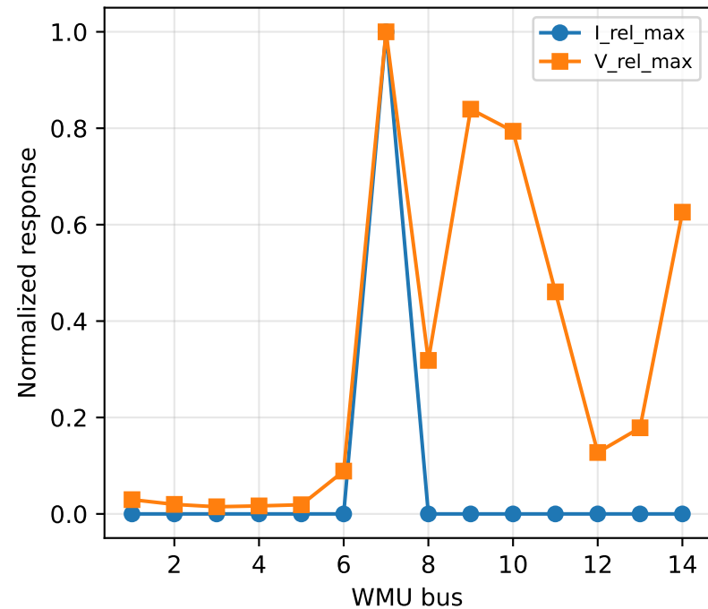
ieee14 representative CaseID 24
