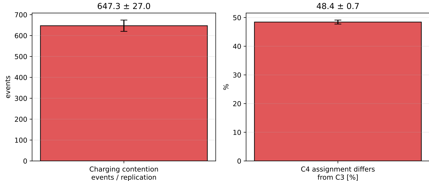
Figure 3. C4 Priority Algorithm behavior verification (mean \pm 95% CI, n=50)
