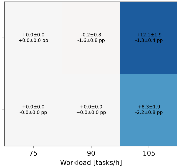
Final Stress Grid: C4 versus C3 (mean \pm 95% CI, n=50)
