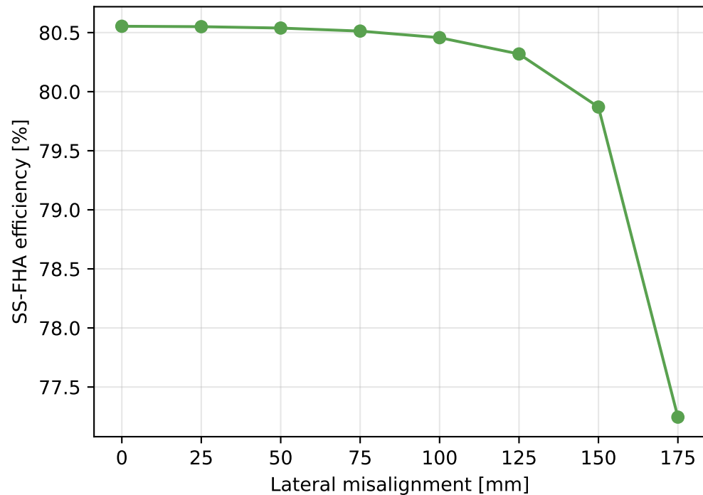
Geometry-derived WPT coupling and SS-FHA efficiency
