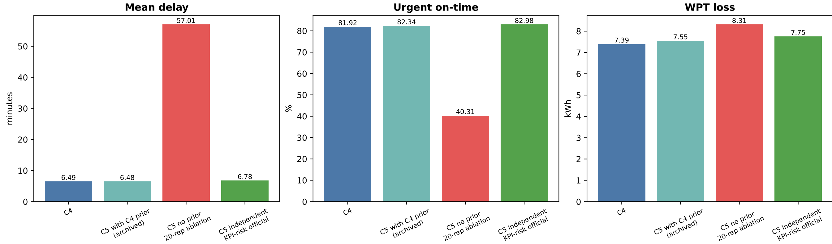
Figure 5. C5 objective ablation: C4-prior dependence and independent KPI-risk replacement
