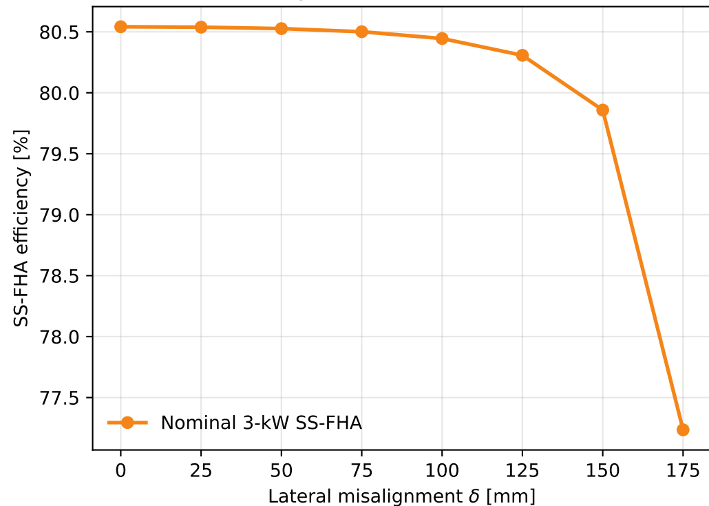
(a) Analytical nominal 3-kW model
