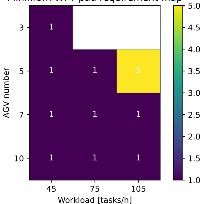
Minimum WPT pad requirement map
