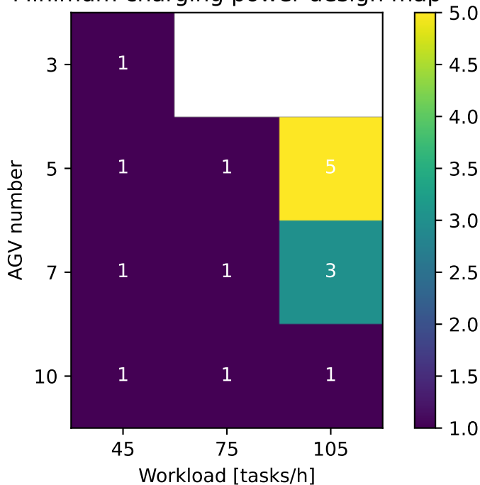
Minimum charging power design map
