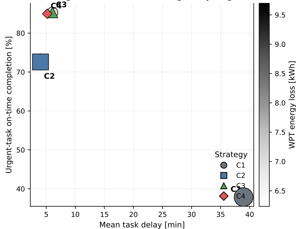
Challenge Case trade-off among delay, urgent service, and WPT loss
