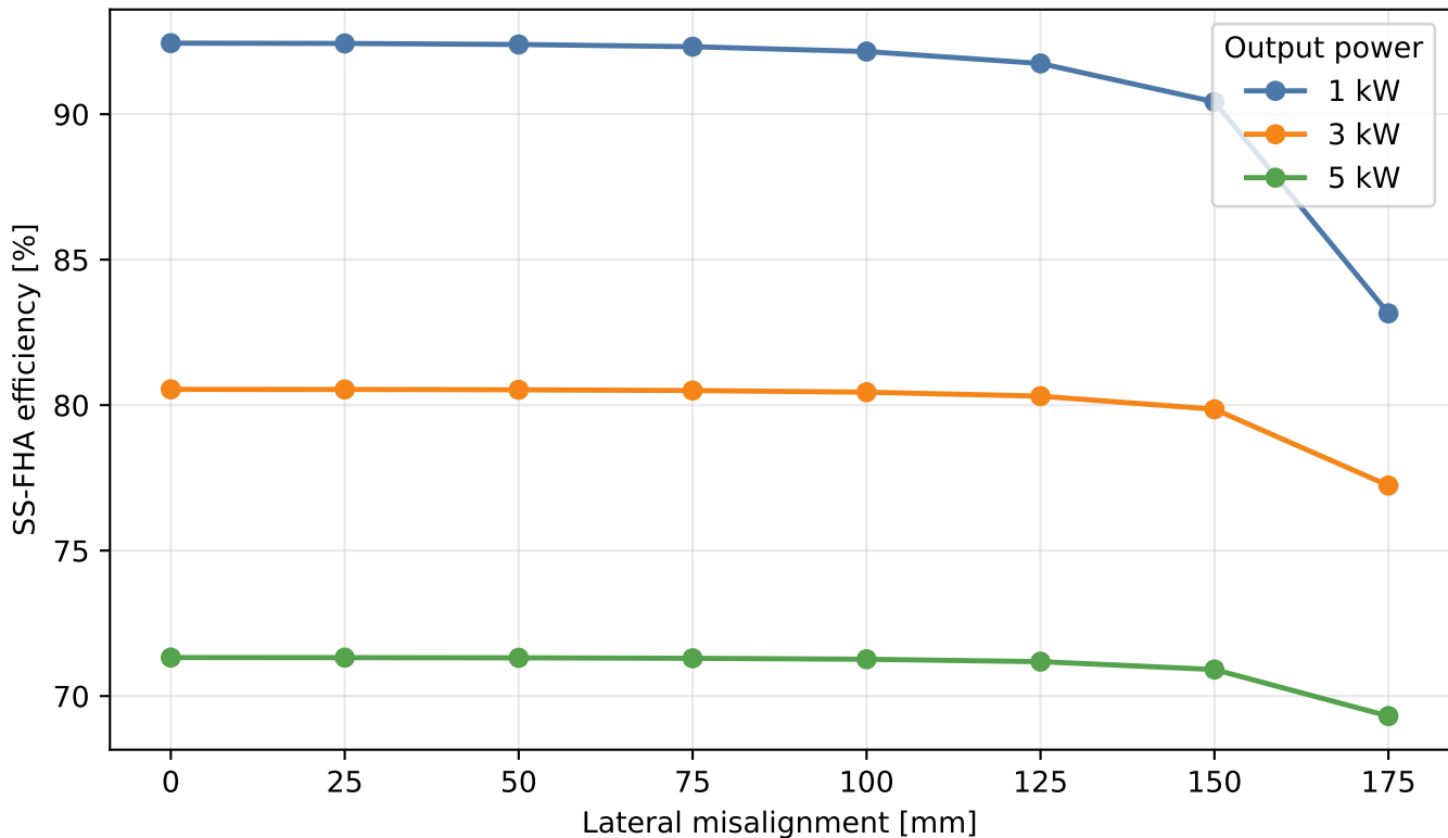
Power-dependent SS-FHA efficiency under 48-V nominal DC-side assumption
