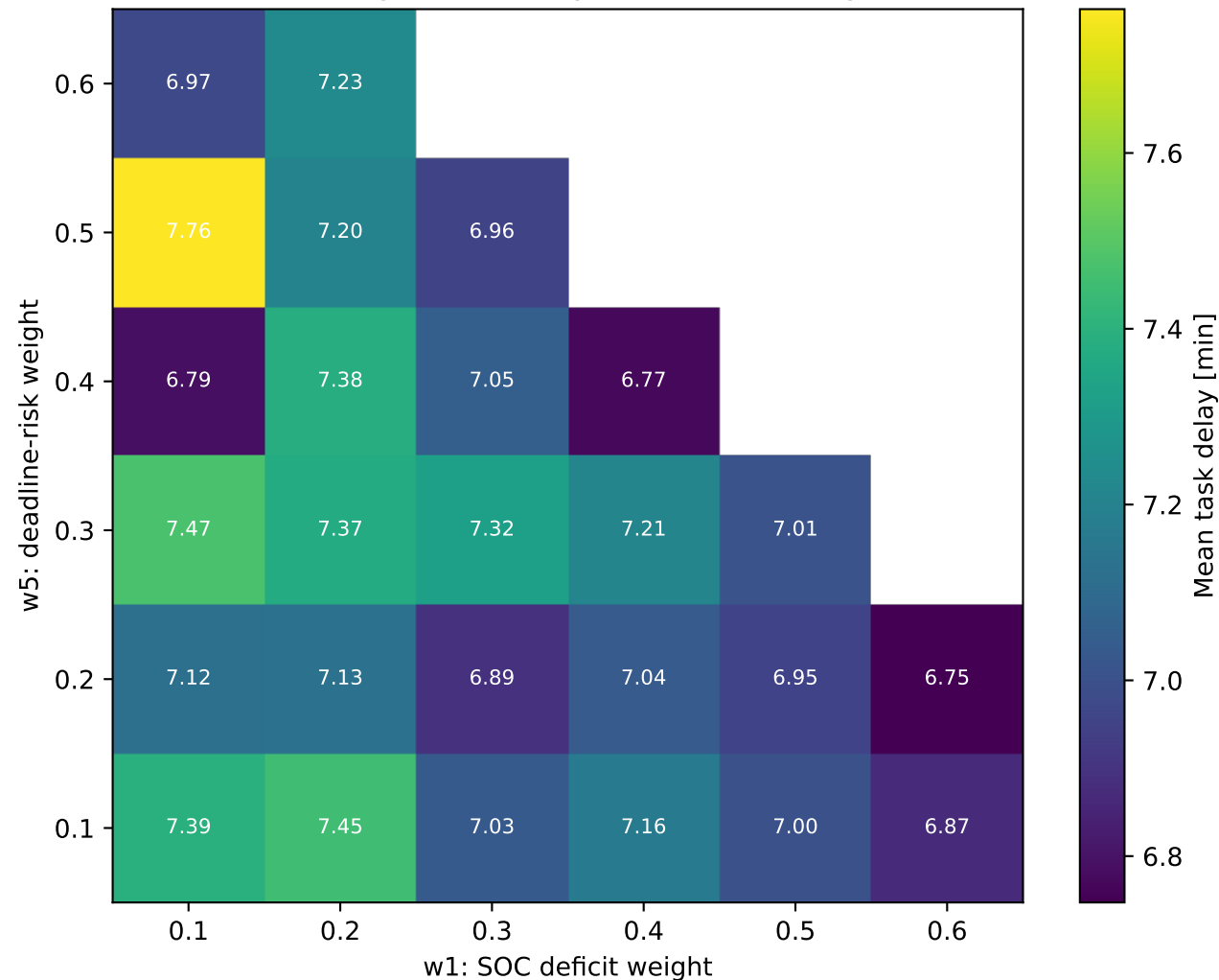
C4 weight sensitivity: mean task delay
