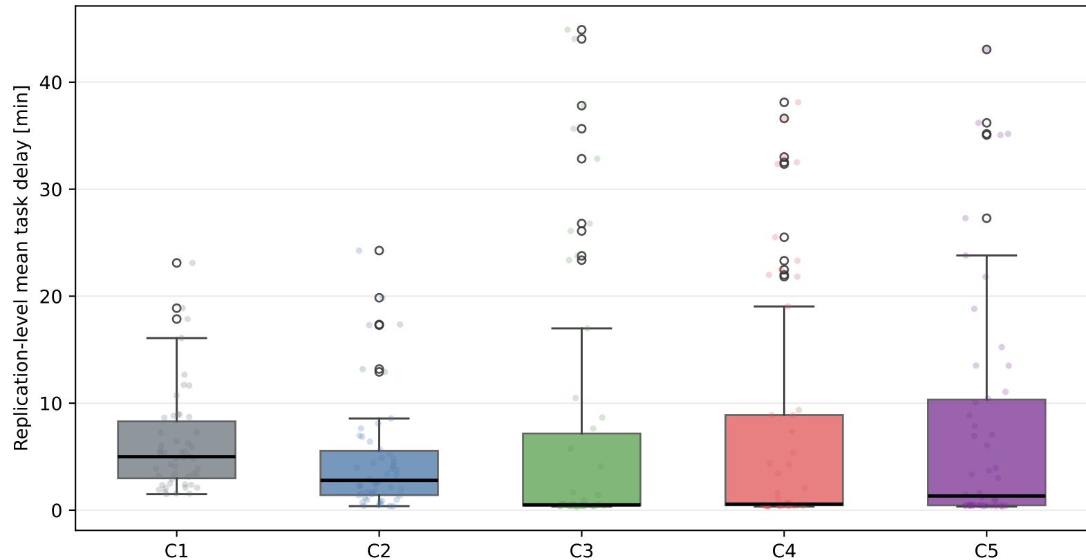
Figure 6. Primary Challenge delay distribution across 50 replications
