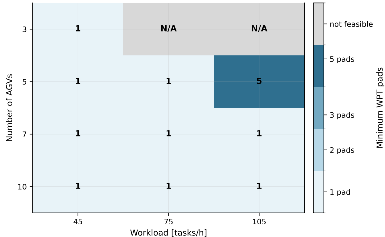
Figure 3. Minimum WPT pad requirement for 99% completion and zero stoppage
