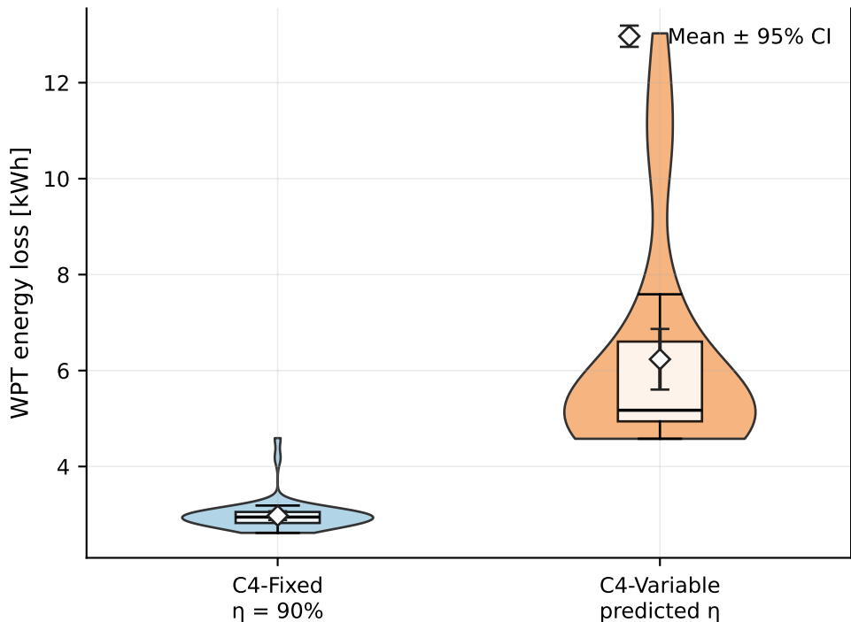
Figure 4. Value of WPT efficiency-aware scheduling in C4 ablation
