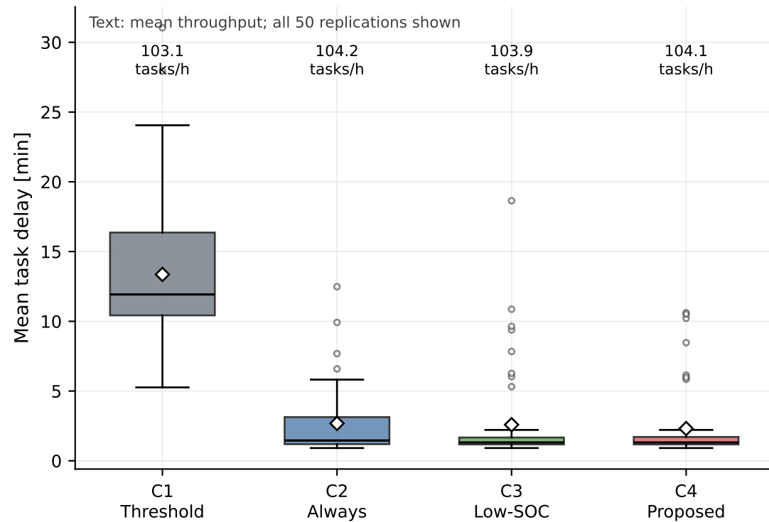
Figure 2. Delay distribution in a C4-advantage stress region (105 tasks/h, 2 pads, 5 kW)
