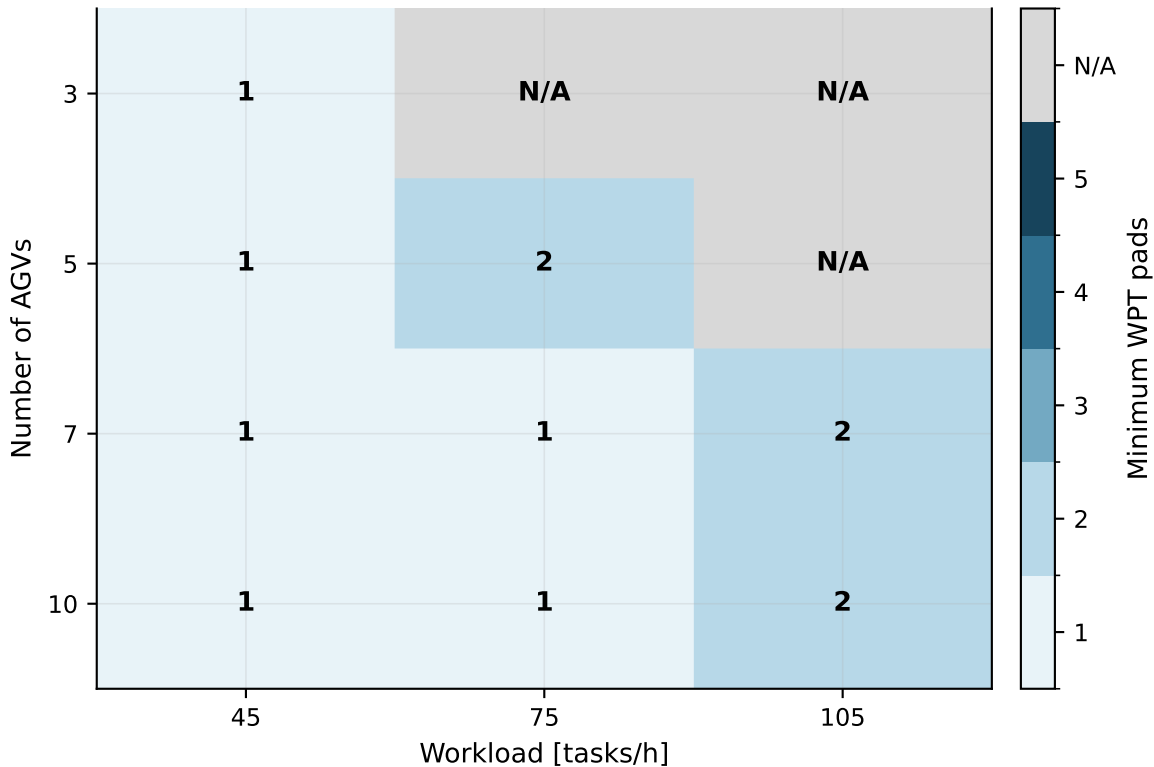
Figure 3. Minimum WPT pads under tightened energy assumptions
