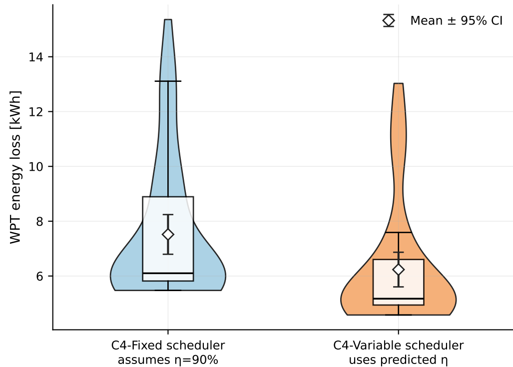
Figure 4. Corrected efficiency ablation: same realized variable \eta , different scheduler knowledge
