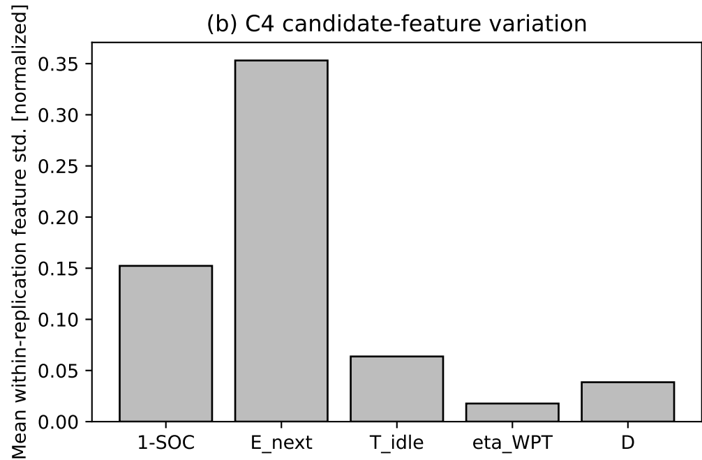
Figure 3. C4 Priority Algorithm behavior verification
