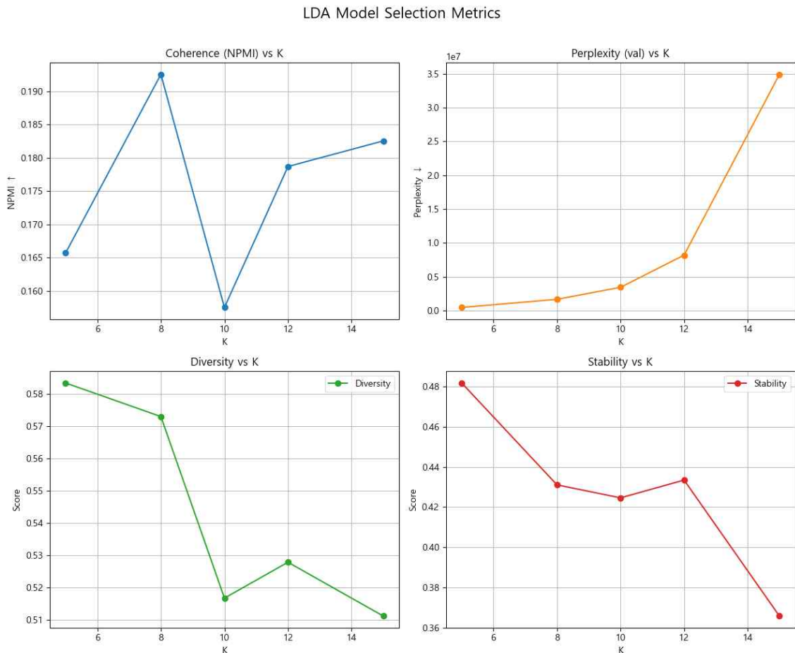
Figure 2. LDA 모델 토픽 수(K)별 Coherence, Perplexity, Diversity, Stability 비교
