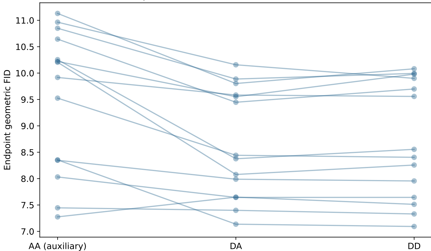
Only common valid AA/DA/DD seeds, n=14
