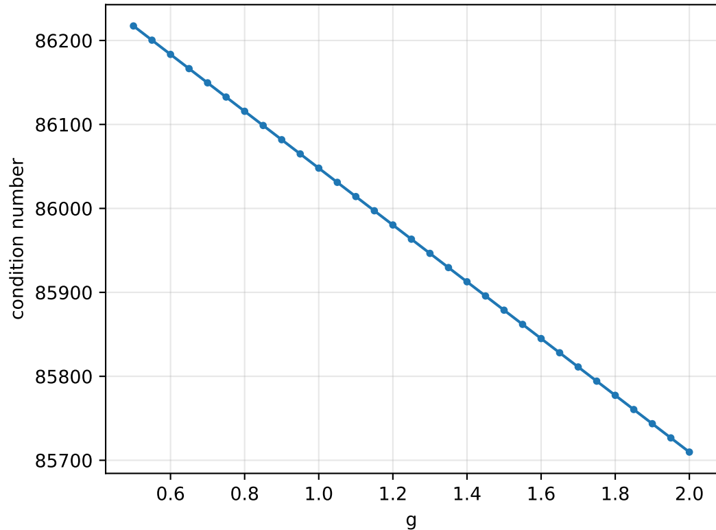
Hessian condition number vs gap scale g
