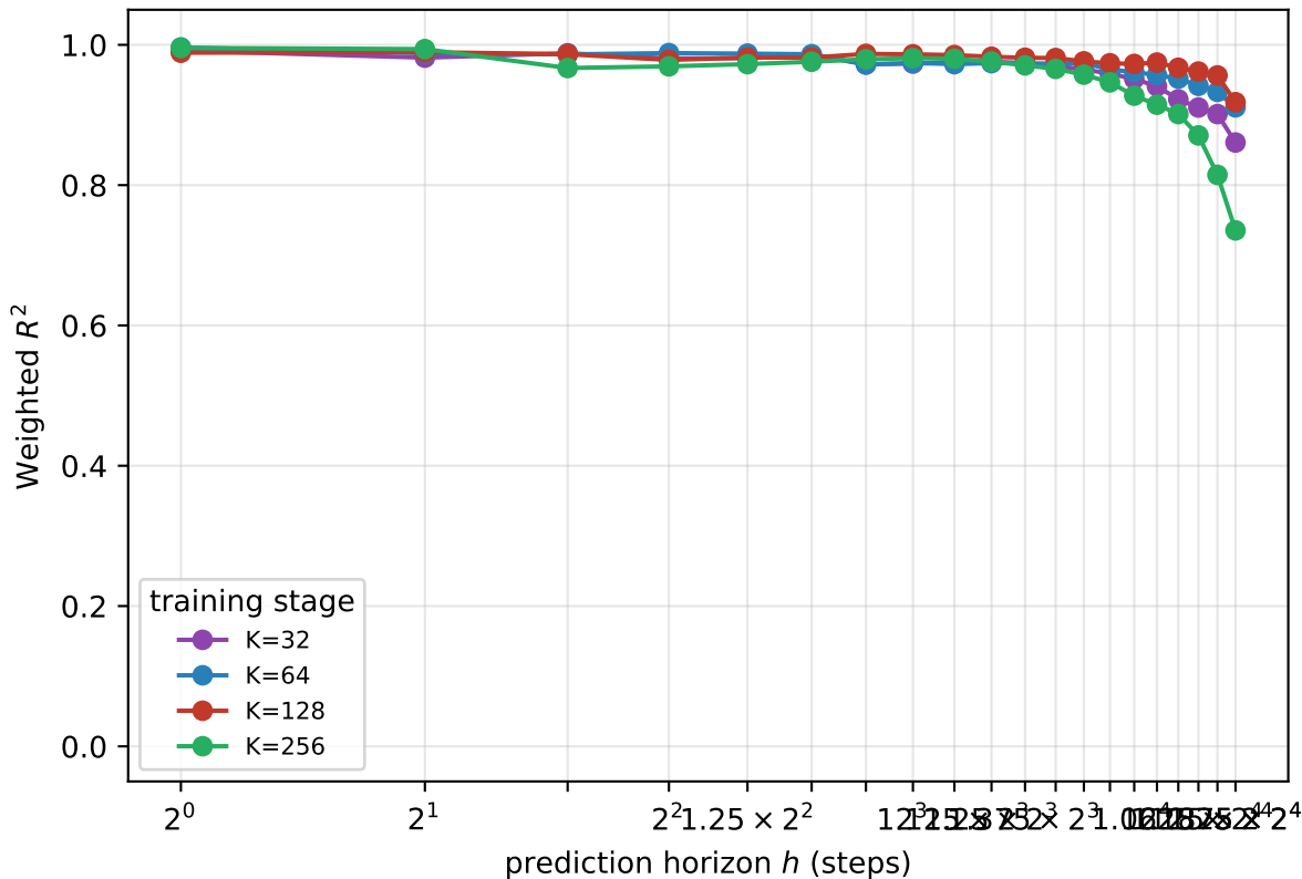
Scalar-history explanatory power vs prediction horizon
