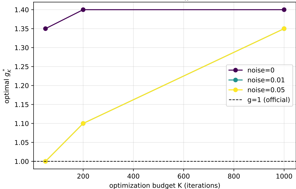
Internal optimal gap g_K^* vs budget
