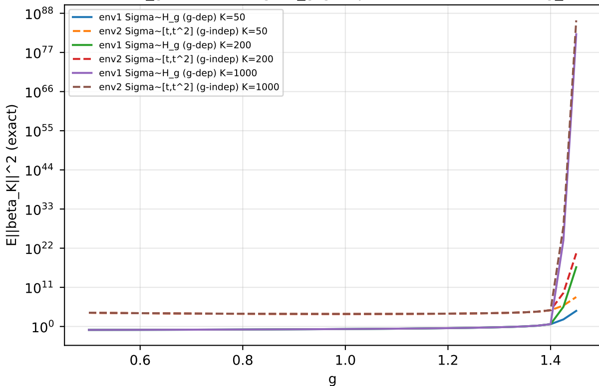
Same H_g , different \Sigma_g(g\text{-dependence}) \rightarrow different g_{K^*}
