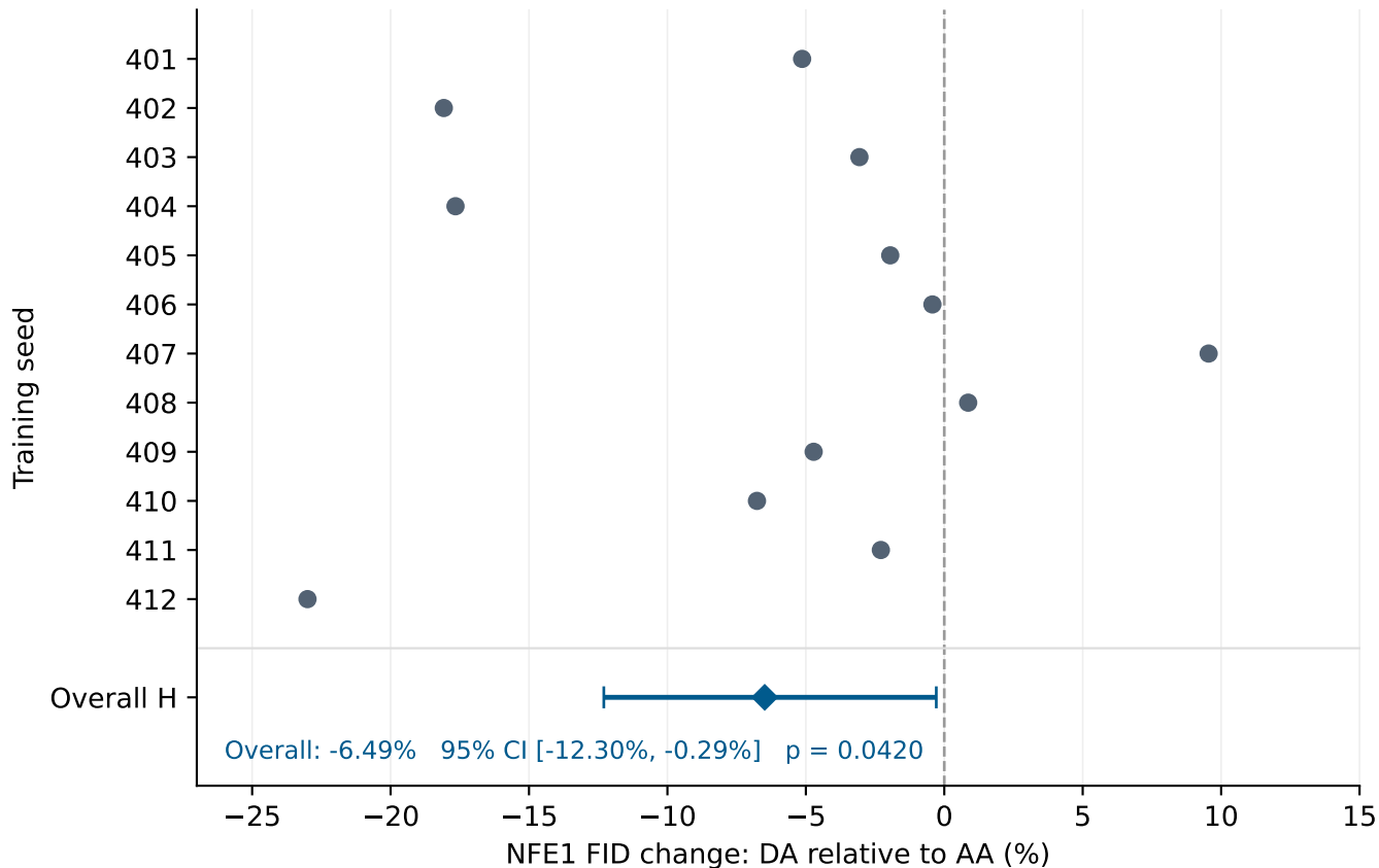
F12 at q = 256: fixed fresh cohort (n = 12)
