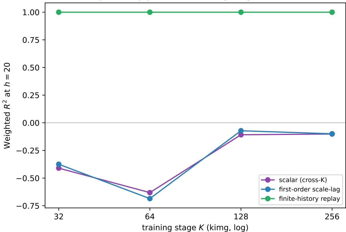
Predictor explanatory power vs training stage (h=20, fresh start)
