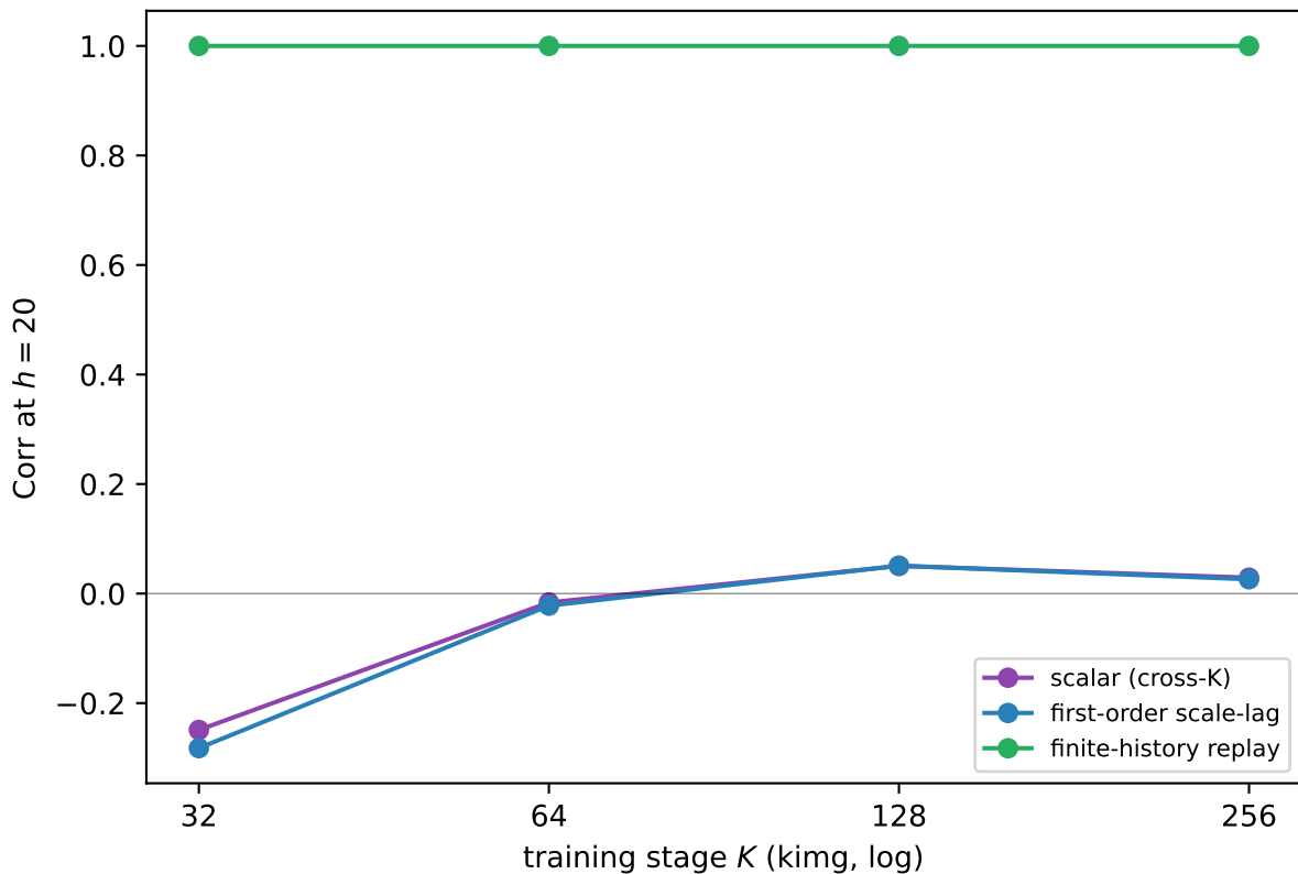
Predictor correlation with actual h vs training stage ( h=20 , fresh start)
