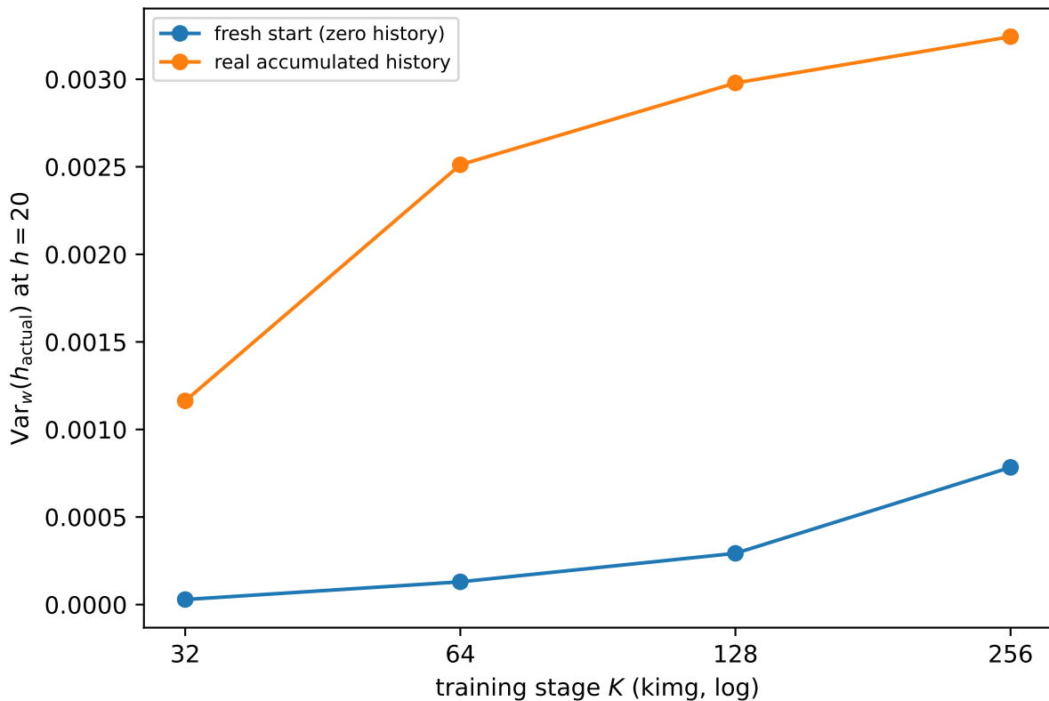
Target variance of the update ratio (contextualizes R^2 )
