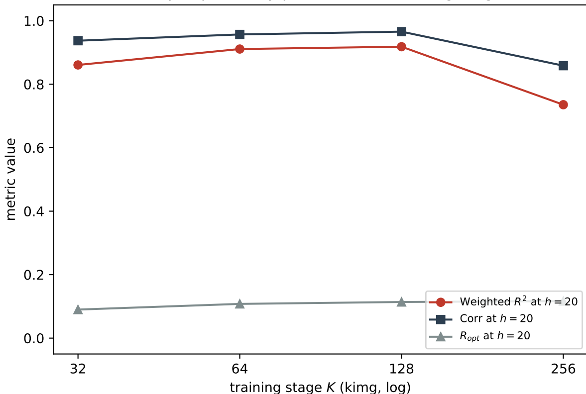
Scalar-history explanatory power across training stages ( h=20 )
