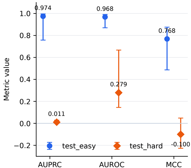
A Performance gap (kmer13 + LR)
