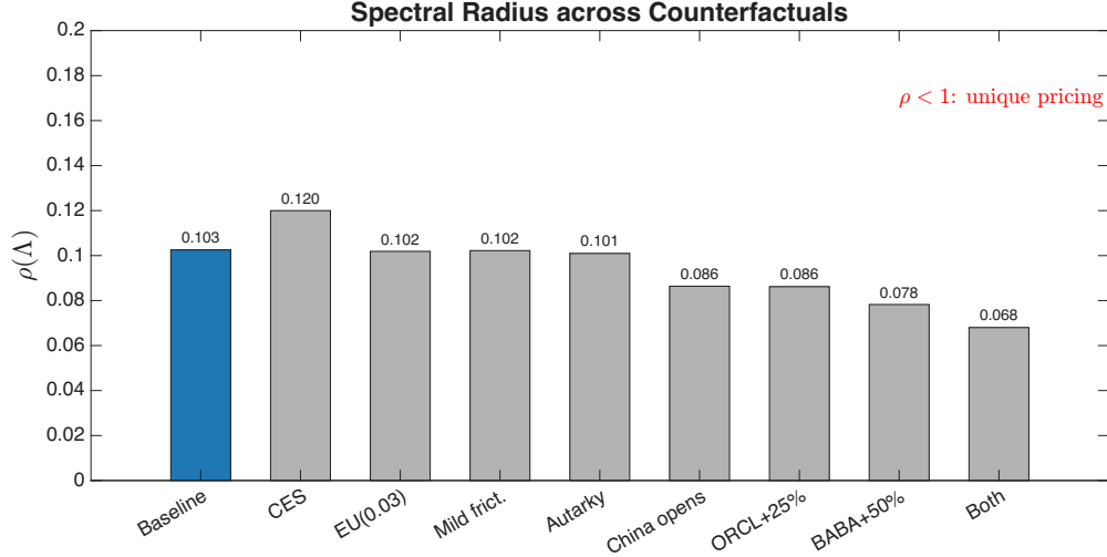
Figure 5: Spectral radius \rho(\Lambda) across all counterfactual scenarios. The baseline and all counterfactuals satisfy \rho(\Lambda) < 0.15 \ll 1 , confirming pricing uniqueness throughout.
