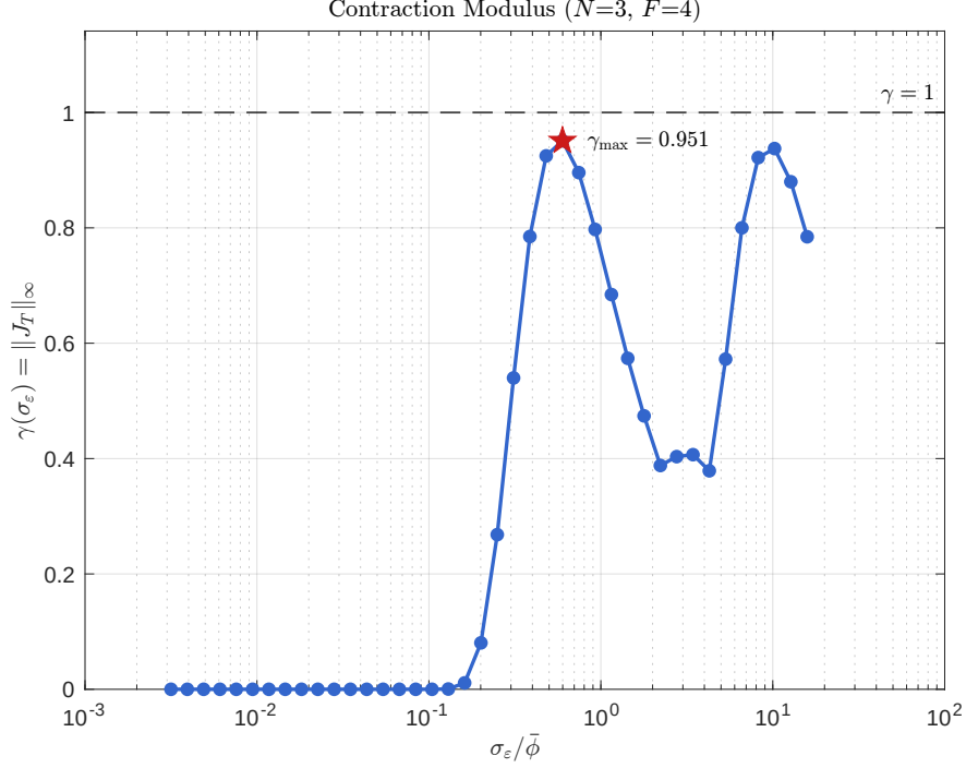
Figure 2: Contraction modulus \gamma(\sigma_\varepsilon) for a small economy ( N = 3, F = 4 ). The bathtub shape confirms Proposition 16(iv): uniqueness tightens at both extremes of the noise scale, and the peak \gamma_{\max} = 0.951 (marked) is below the \gamma = 1 threshold. See Appendix F for scaling across economy sizes.
