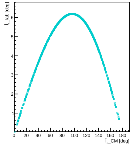
Lab Angle vs CM Angle
