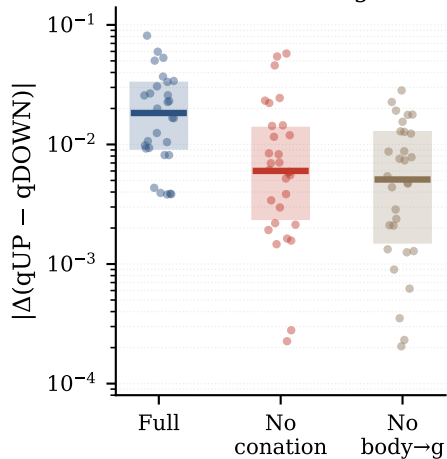
(c) Readiness-shift magnitude
