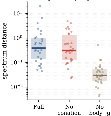
(b) Metric-geometry separation
