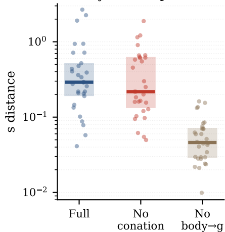
(a) Policy-state separation
