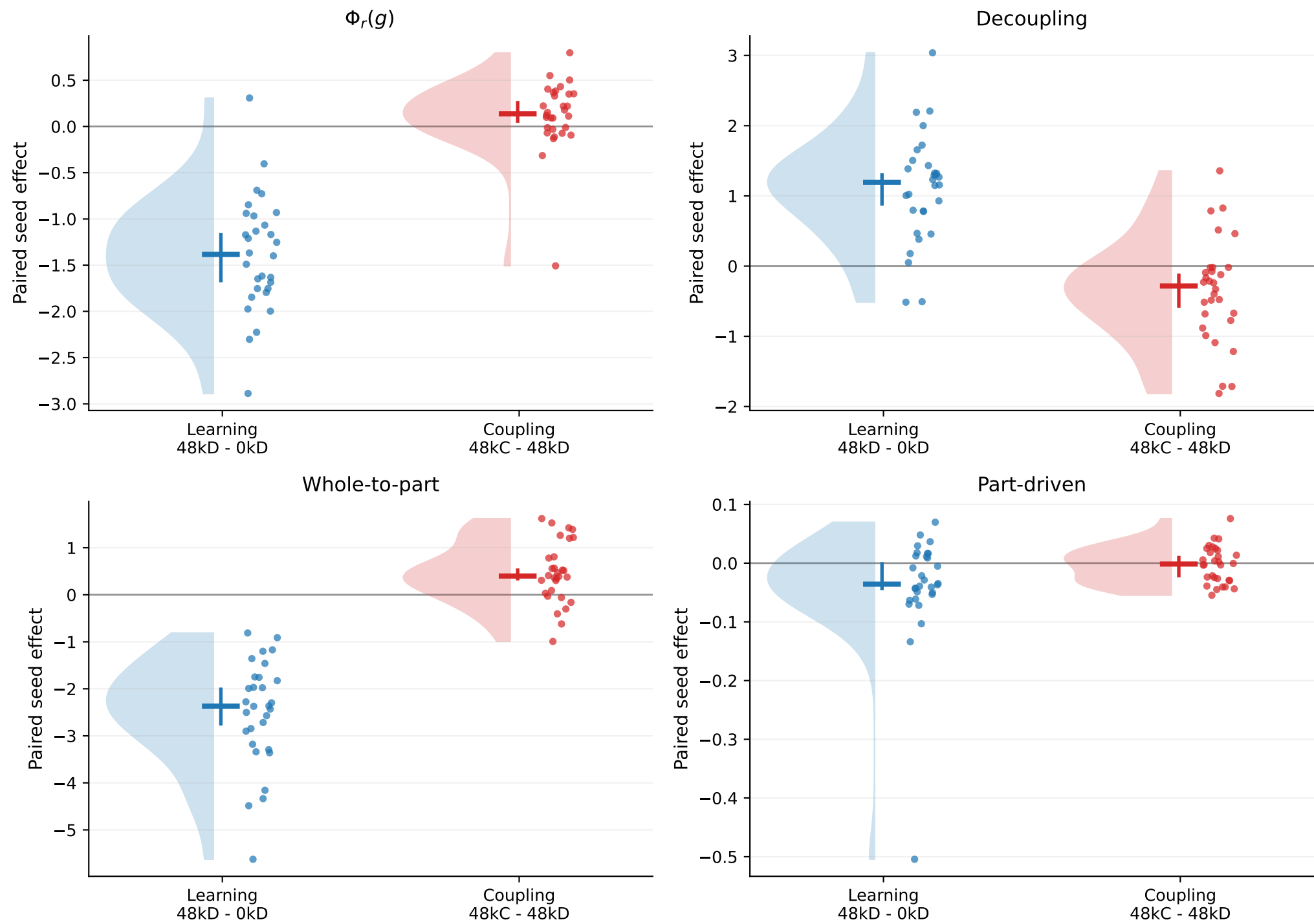
Figure 4. Paired effects of learning and policy-side gradient coupling
