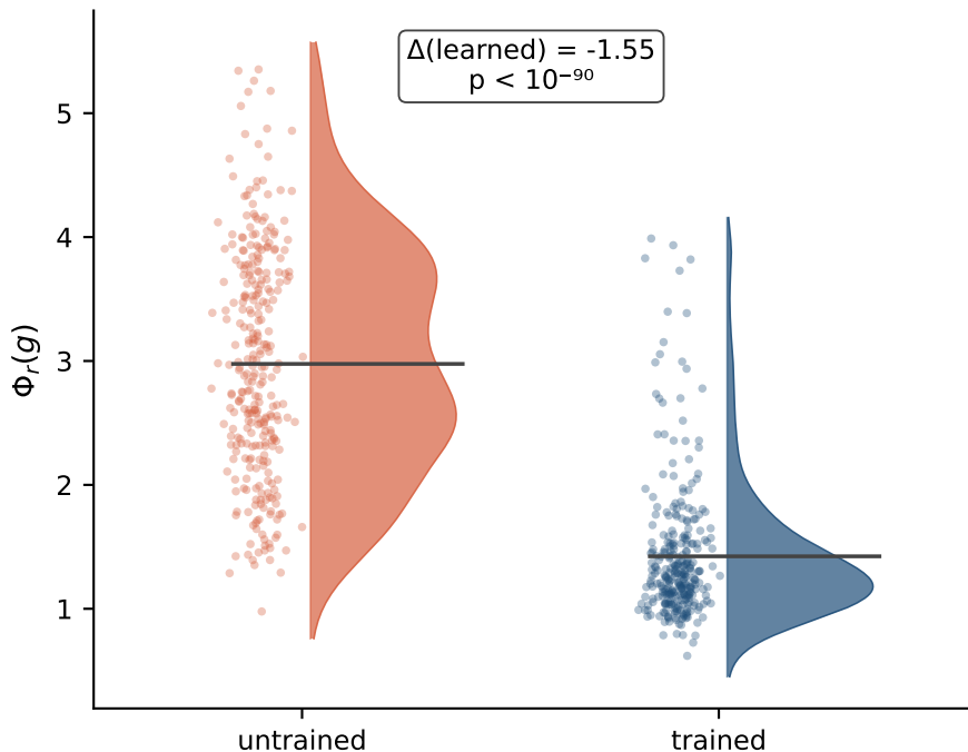
Magnitude: untrained vs trained (clean)
