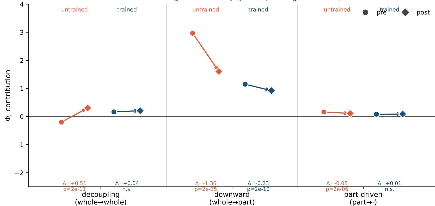
Atom-level regime sensitivity (pre \rightarrow post regime switch)
