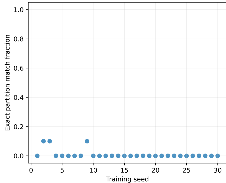
48k default-coupled Fiedler partition diagnostics
