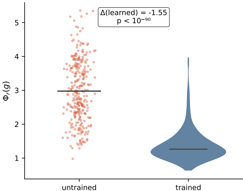
Magnitude: untrained vs trained (clean)
