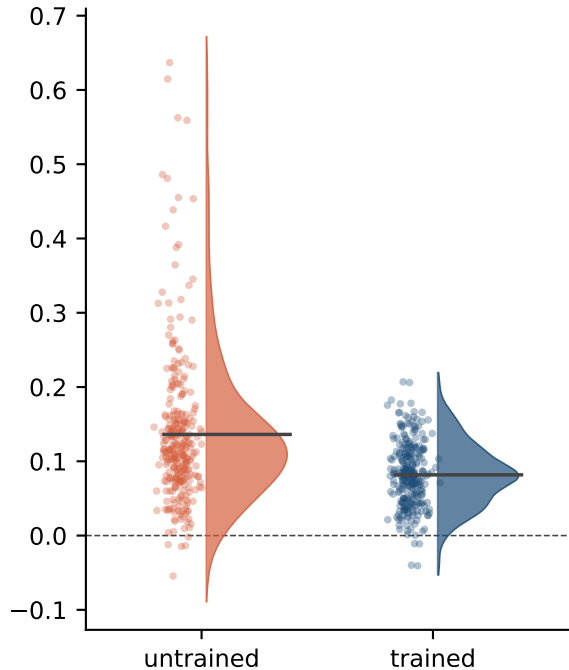
(c) part-driven (part \rightarrow part) untrained: +0.14 | trained: +0.08
