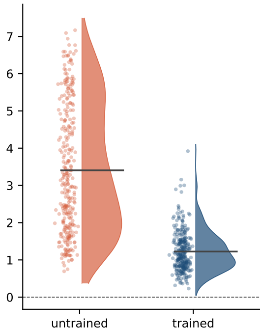
(b) downward (whole \rightarrow part) untrained: +3.41 | trained: +1.22
